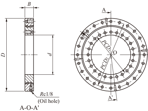
Fig. 5 Manufacturing example
