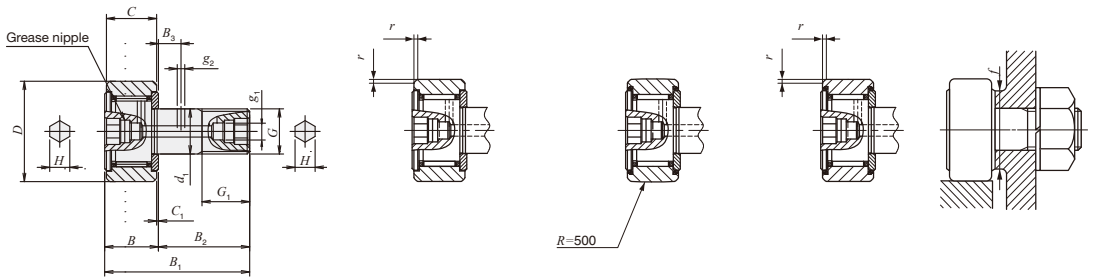
Outside dia. of outer ring D 30 - 90 mm CFKR CFKR...UUR CFKR...UU
