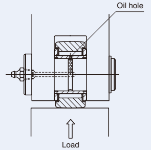
Fig. 2 Position of oil hole and load direction
